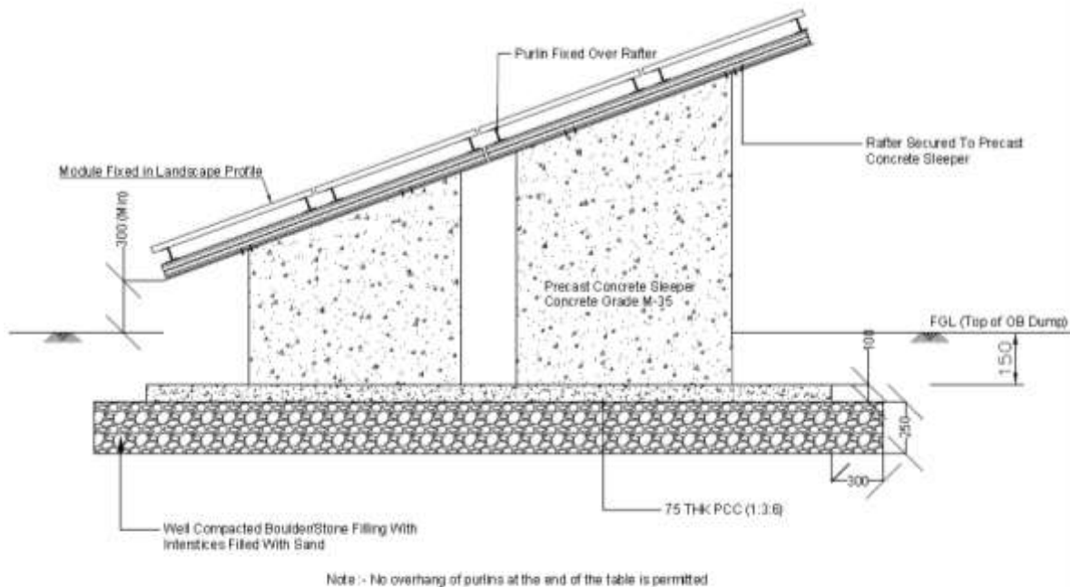
Schematic Details of MMS Structure & Support Precast RCC Sleeper
